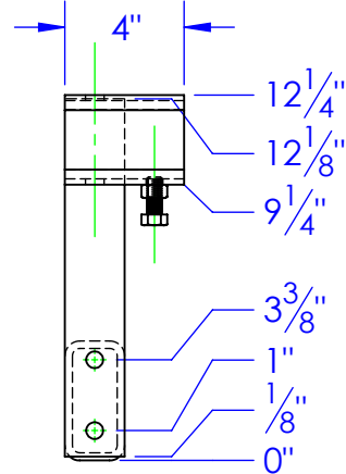
OP-PIPE H-PS 150 FRONT PS
