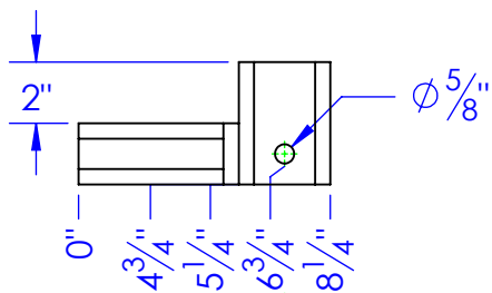
OP-PIPE H-PS 150 FRONT PS
