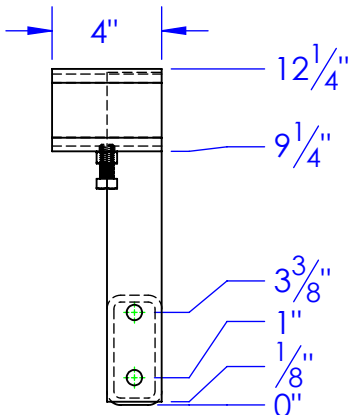
OP-PIPE H-PS150 FRONT
